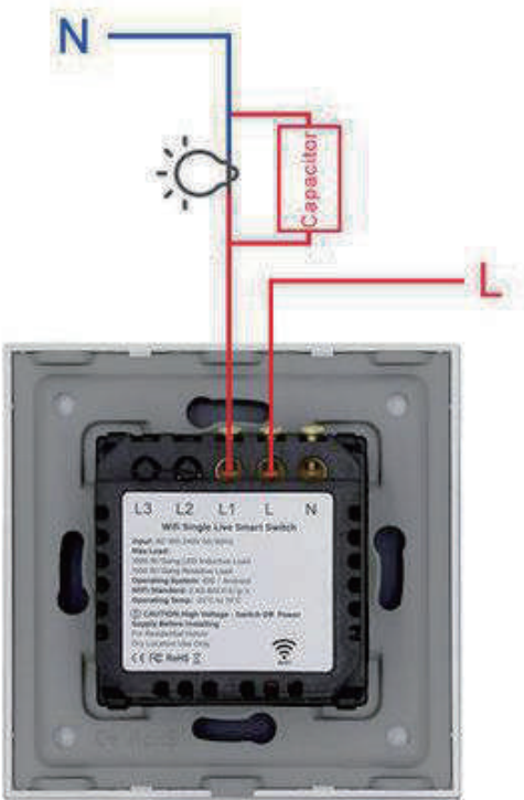
Wiring Diagram
